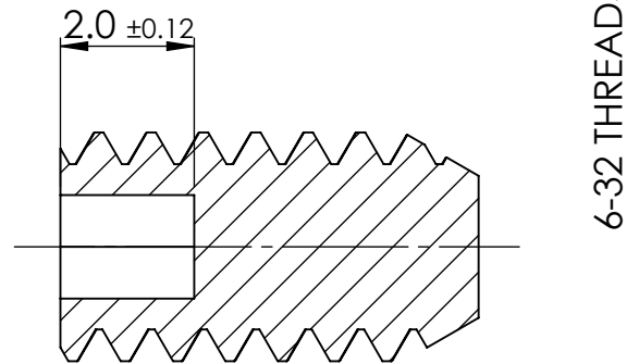
SECTION X-X
